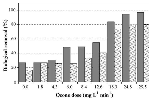
Fig. 2. Removal percentages of DOC (grey bars) and organic nitrogen (dotted bars) in the biological assays performed with the effluent ozonated at different ozone doses.
