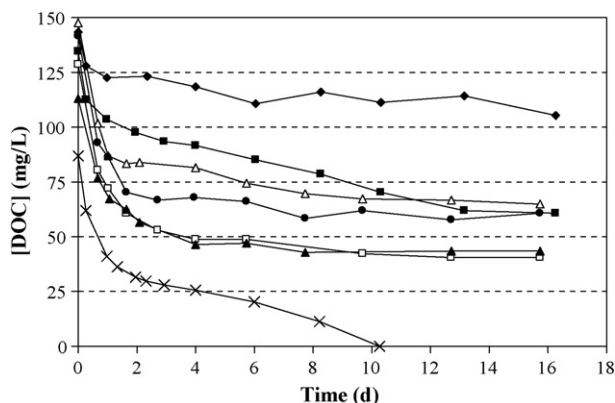
Fig. 3. DOC evolution in the biological assays performed with the effluent ozonated at different ozone contact times: without ozonation (◆), 30 min (■), 45 min (△), 60 min (●), 90 min (□), 120 min (▲) and 180 min (×).
