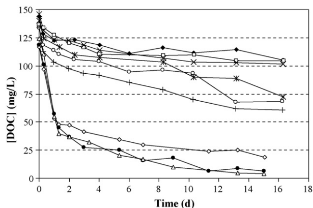
Fig. 1. DOC evolution in the biological assays performed with the effluent ozonated at different ozone doses: without ozonation ( \blacklozenge ), 1.8 \text{ mg L}^{-1} \text{ min}^{-1} ( \square ), 4.3 \text{ mg L}^{-1} \text{ min}^{-1} ( \times ), 6.0 \text{ mg L}^{-1} \text{ min}^{-1} ( \otimes ), 8.4 \text{ mg L}^{-1} \text{ min}^{-1} ( \circ ), 12.6 \text{ mg L}^{-1} \text{ min}^{-1} ( + ), 18.3 \text{ mg L}^{-1} \text{ min}^{-1} ( \diamond ), 24.8 \text{ mg L}^{-1} \text{ min}^{-1} ( \bullet ) and 29.5 \text{ mg L}^{-1} \text{ min}^{-1} ( \triangle ).
