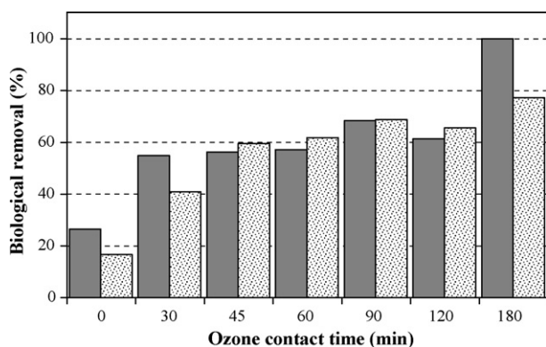
Fig. 4. Removal percentages of DOC (grey bars) and organic nitrogen (dotted bars) in the biological assays performed with the effluent ozonated at different ozone contact times.
